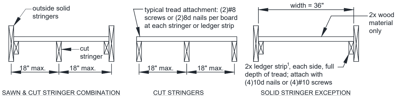
FIGURE 42: STRINGER TREADS
